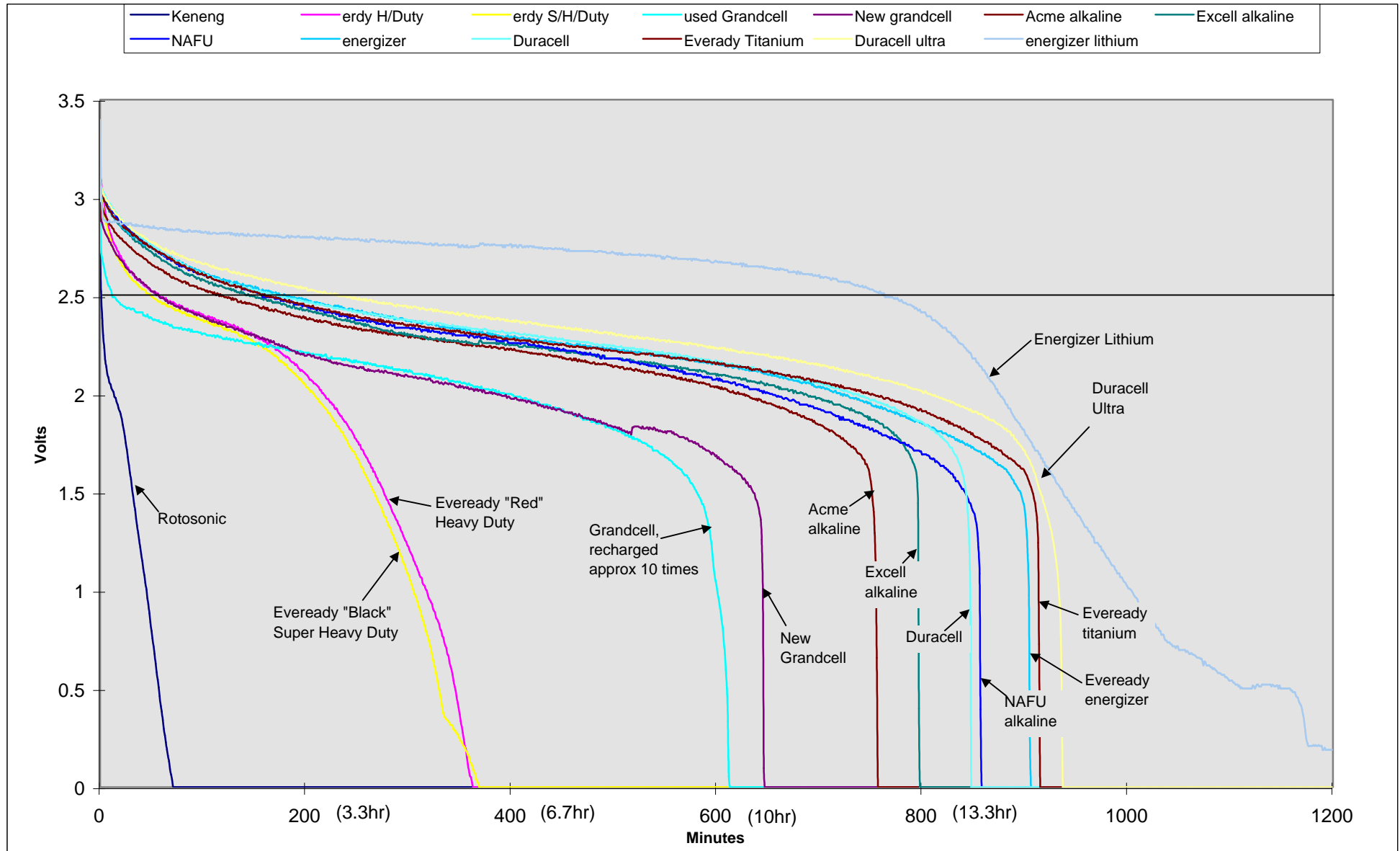
AA batteries at 160mA load Chart 4
