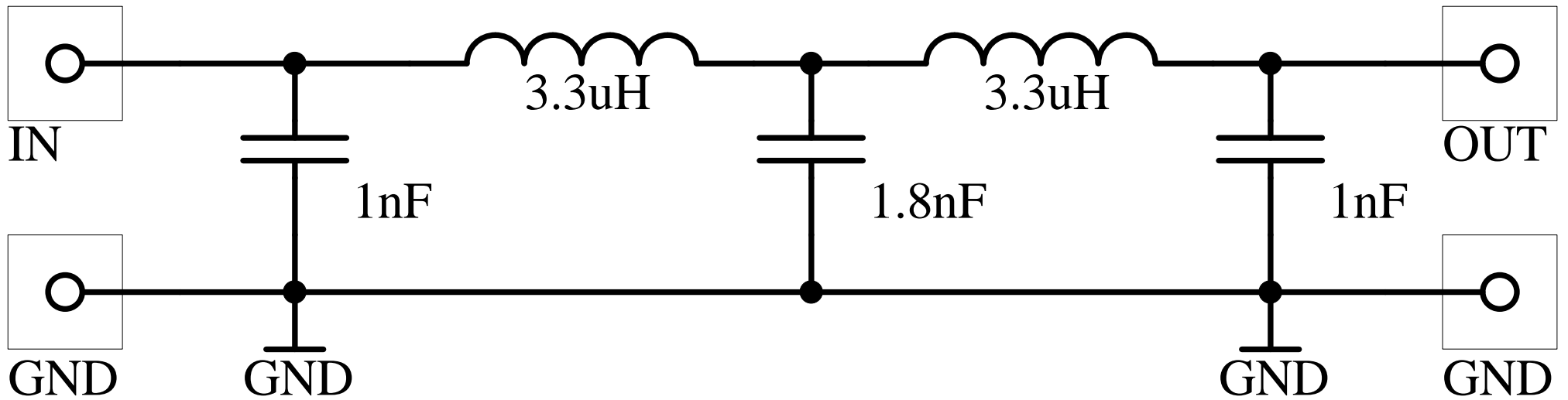
Figure 4 - 3.5MHz Low Pass Filter
