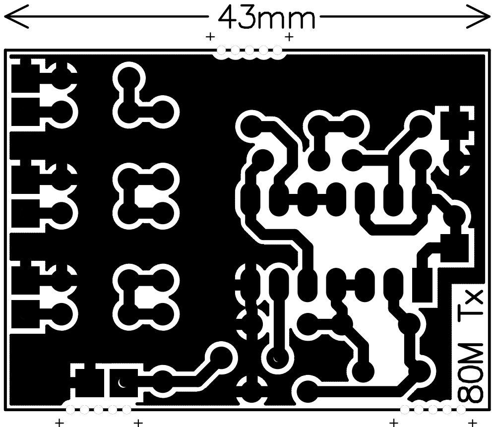
Figure 3 – PCB Artwork
