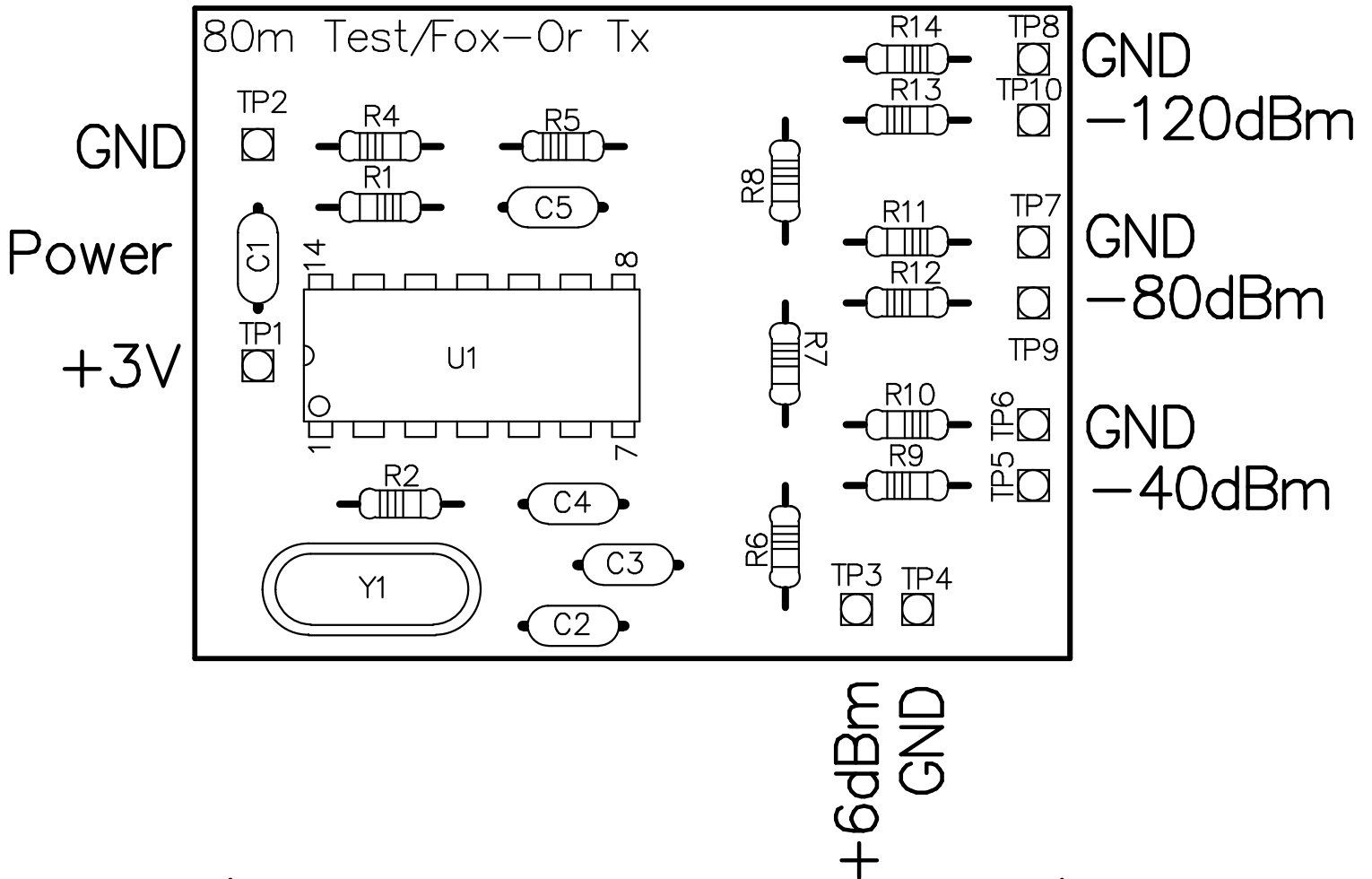
Figure 2 – Component mounting
