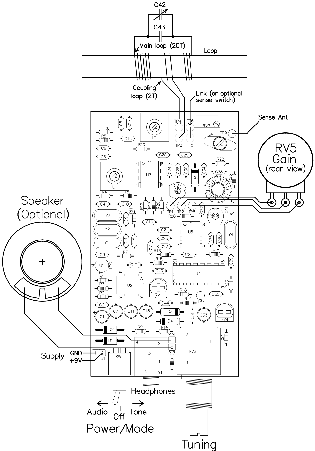
Figure 5 – Board loading and external connections
